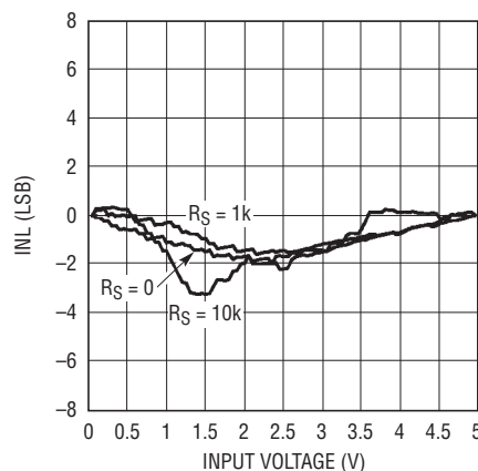
Figure 17. Measured INL vs V_{IN} , C_{IN} = 0 , V_{CC} = 5V , T_A = 25^\circ C
