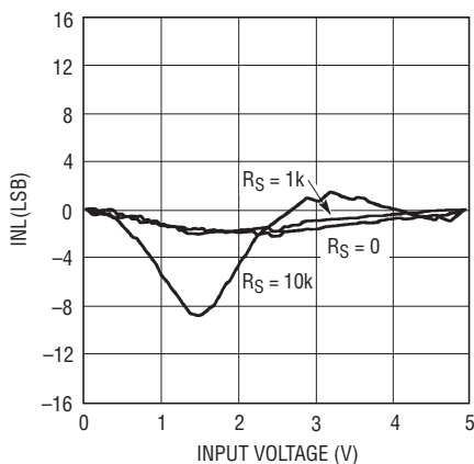
Figure 16. Measured INL vs Input Voltage, C_{IN} = 0.1\mu F, V_{CC} = 5V , T_A = 25^\circ C
